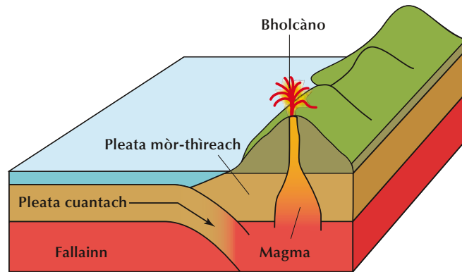
Diagram 11.16: Crìoch-pleata millteach
