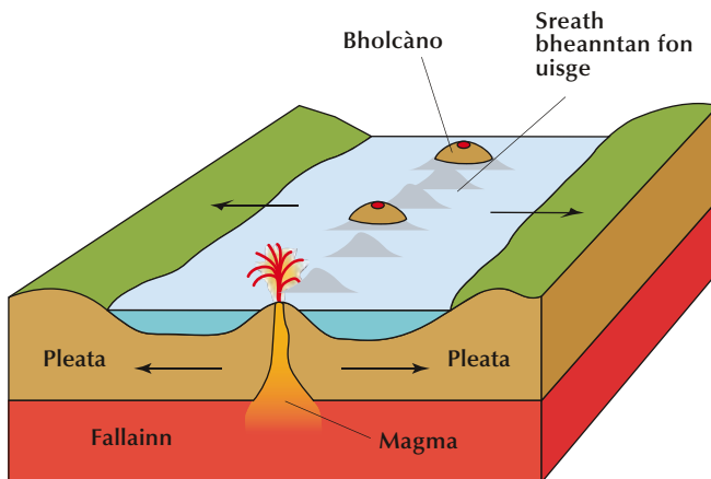
Diagram 11.15: Crìoch-pleata constructach
