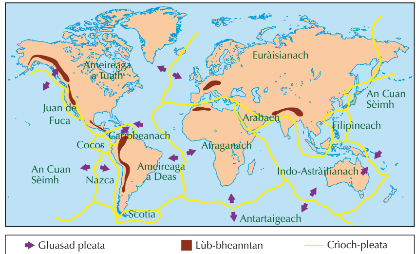
Diagram 11.3: Pleataichean teactonaig
