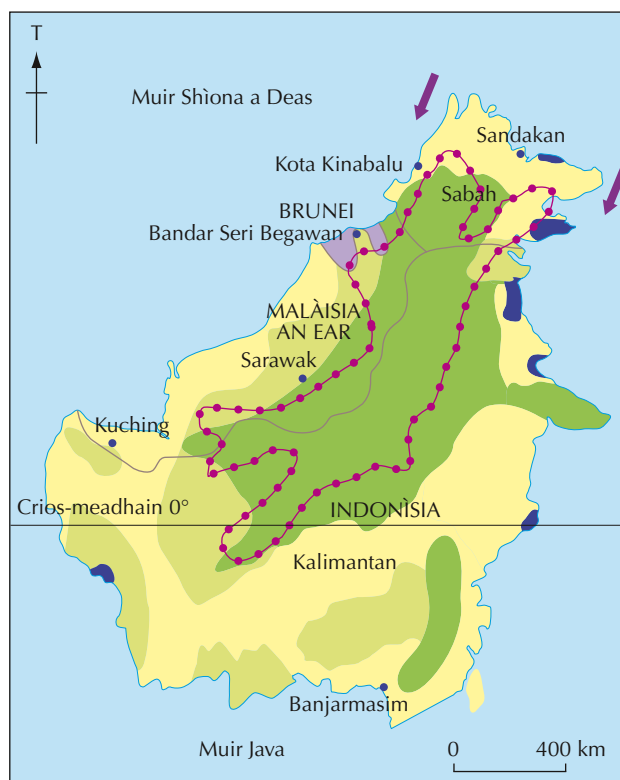
Diagram 12.8: Eilean Bhorneo
