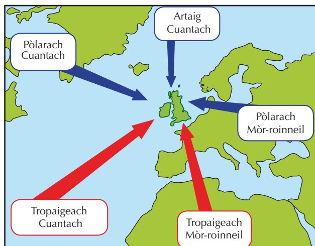
Diagram 2.4: Tomadan èadhair
