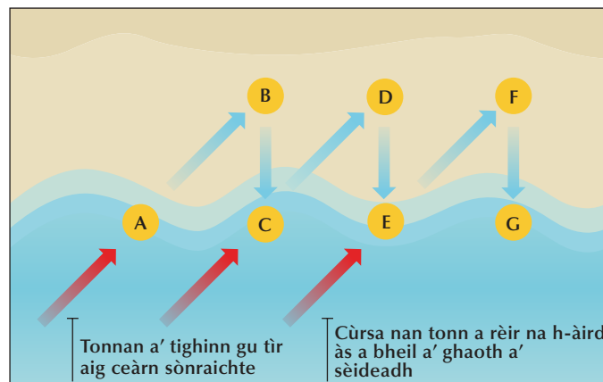
Diagram 6.8: Drioftadh fad-cladaich
